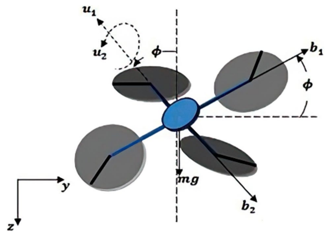
Fig. 1 Quadrotor configuration design
