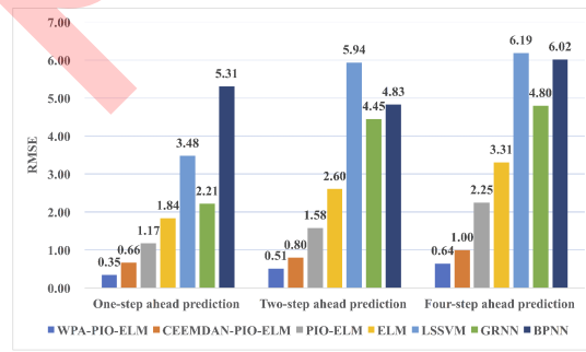
Figure 6 RMSE of WTI Crude oil futures prediction
