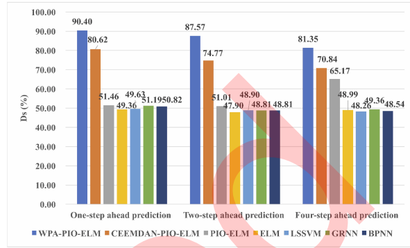
Figure 10 Ds of WTI Crude oil futures prediction
