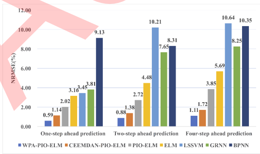
Figure 7 NRMSE of WTI Crude oil futures prediction
