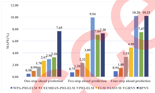
Figure 5 MAPE of WTI Crude oil futures prediction
