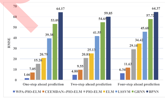
Figure 13 RMSE of CBOT soybean futures prediction
