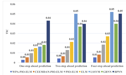
Figure 8 TIC of WTI Crude oil futures prediction
