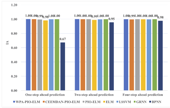
Figure 9 IA of WTI Crude oil futures prediction
