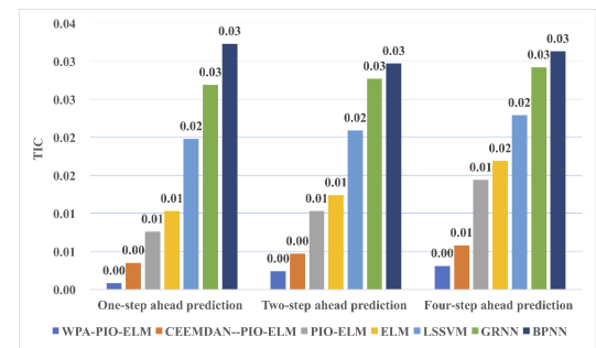
Figure 15 TIC of CBOT soybean futures prediction
